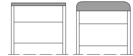
1-mm edge, squared (Carcass furniture)
